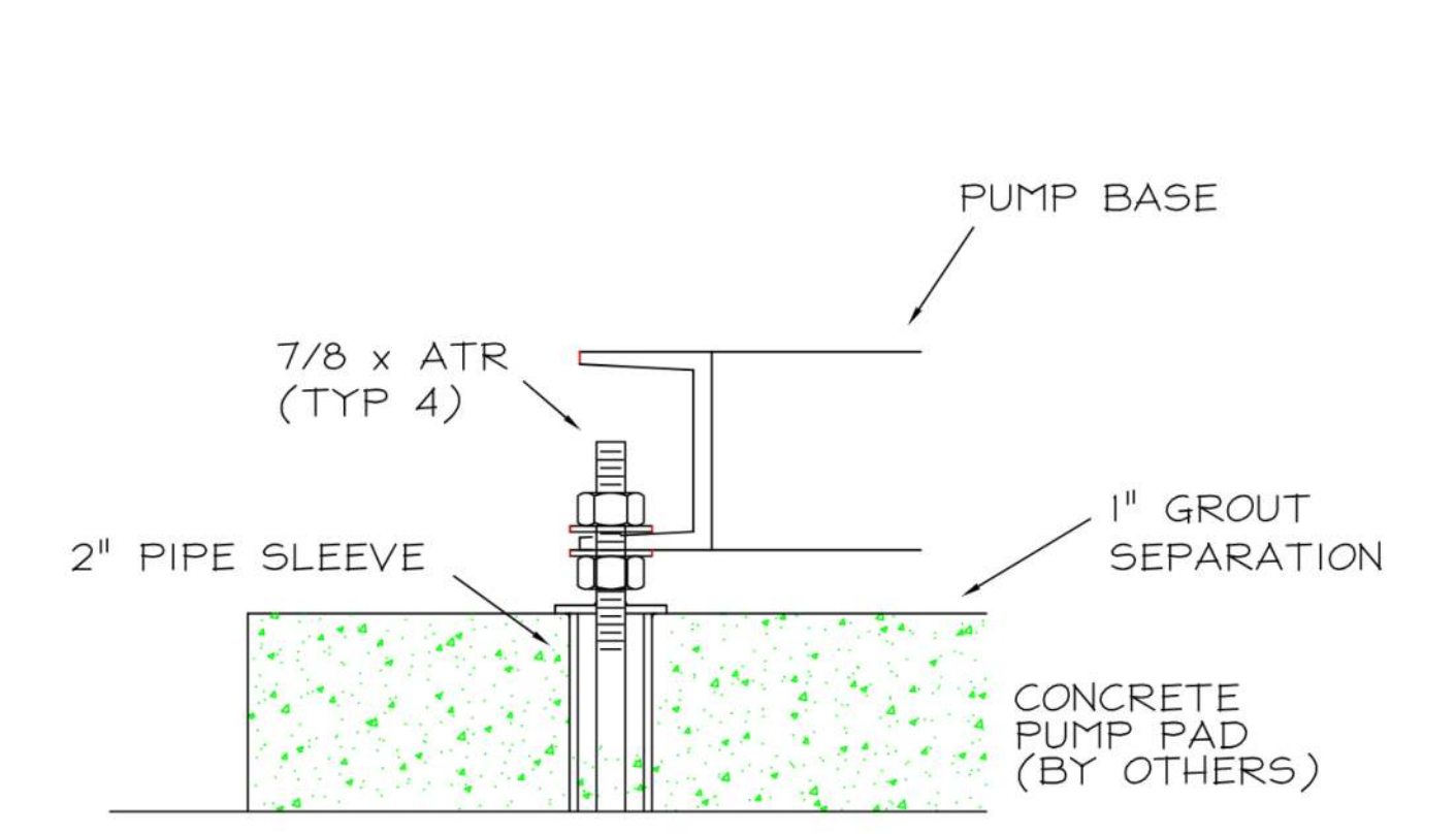
ANCHOR DETAIL NO SCALE
